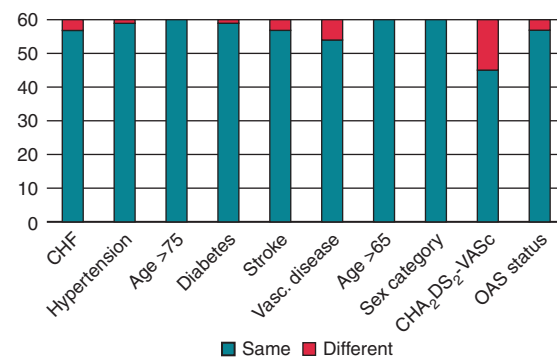
Figure 3 Evaluation of CHA 2 DS 2 -VASc items, total score, and anticoagulation status inferred by AKENATON vs. reference.
