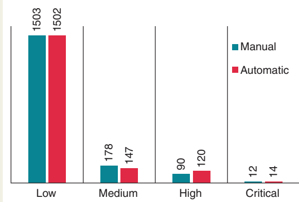
Figure 2 Distribution of AF alert importance classified by human (manual) vs. AKENATON (automatic).
